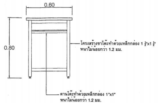
SIDE VIEW Scale 1:20
