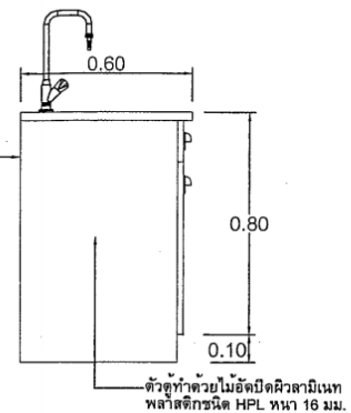
SIDE VIEW Scale 1:20
