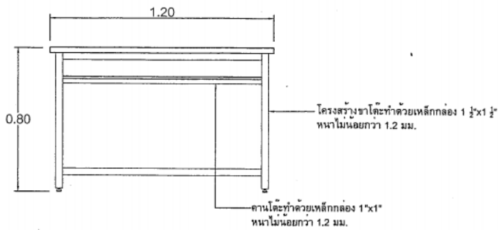
FRONT VIEW Scale 1:20
