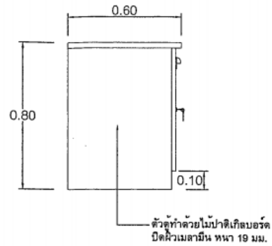
SIDE VIEW Scale 1:20
