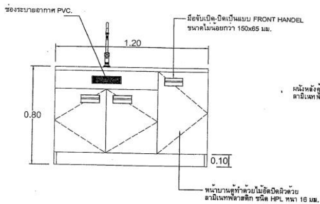
FRONT VIEW Scale 1:20
